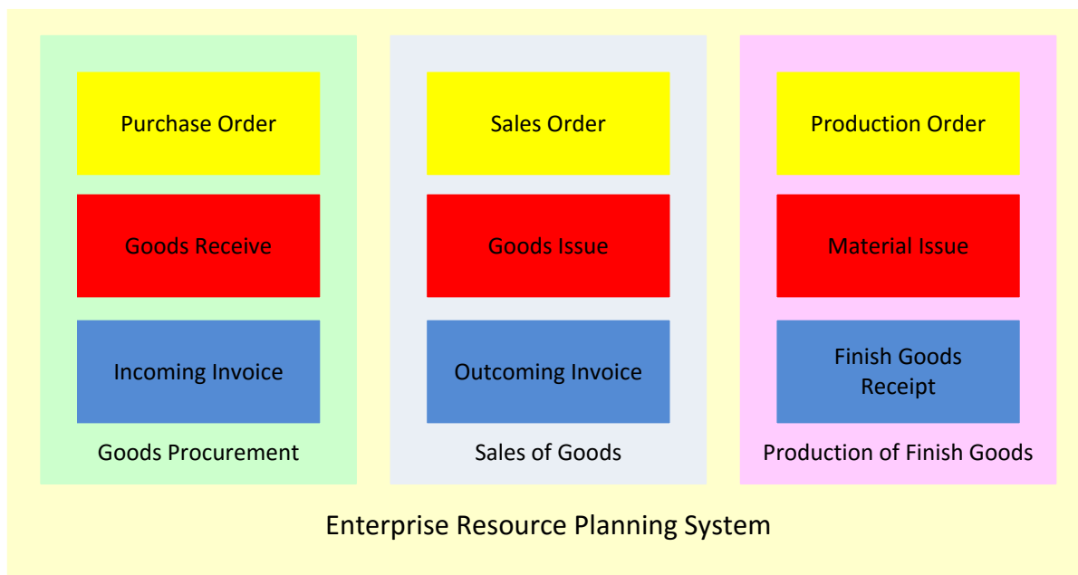
Figure 2. ERP-system architecture
